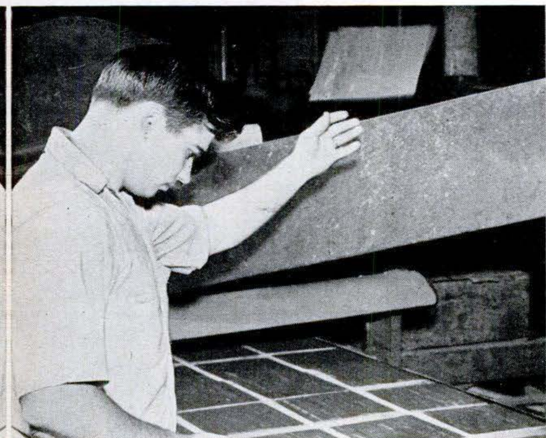
5 A CUTTING MACHINE , using special dies made by Kentile, makes several nine-inch squares at one cut. Inspector watches for imperfect tiles, which are sent back to the Banbury mixer. Refrigerated steel belt further cools tile on way to packing department.
